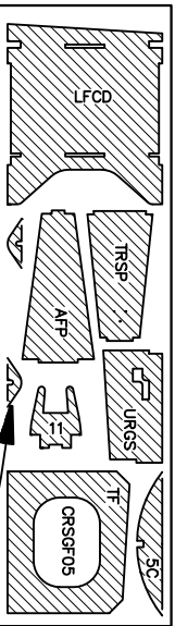
1/8" X 4-1/8" X 27" PLY
